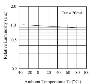
Ambient Temperature vs. Relative Luminescence
